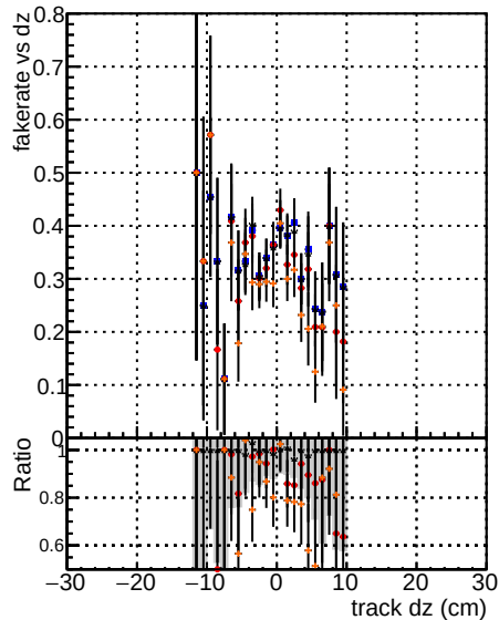
Fake rate vs d DCM mkFit TTbase DCM mkFit 15 TTbase DCM mkFit 16 TTbase trainOldFiles125 v2 prelimWP epoch4 baseline file trainOldFiles125 v2 prelimWP epoch2 wSQCD
