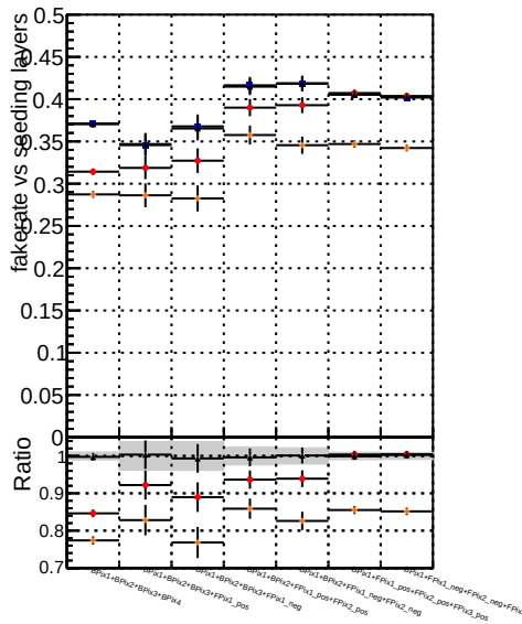
Fake rate vs. DCM mkFit TTbase 5 TTbase retrainOldFiles125_v2 prelimWP epoch4 DCM mkFit 5 TTbase retrainOldFiles125_v2 prelimWP epoch2 wSQCD
