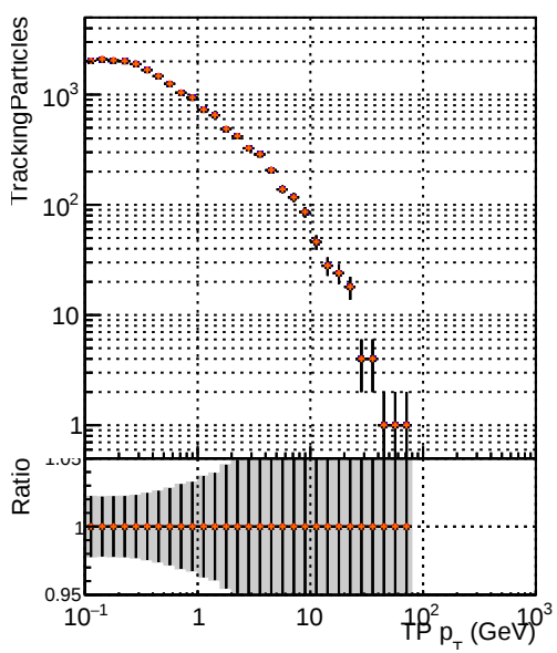
—●— DQM_mkFit6_TT_base —●— DQM_mkFit5_TT_retrainOldFiles125_v2_prelimWP_epoch4 —●— DQM_mkFit6_TT_base —●— DQM_mkFit6_TT_retrainOldFiles125_v2_prelimWP_epoch2_wsQCD
