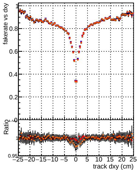
Fake rate vs dxy Duplicates Rate vs Dxy Pileup rate vs dxy Fake rate vs dz Duplicates Rate vs Dxy Pileup rate vs dz
