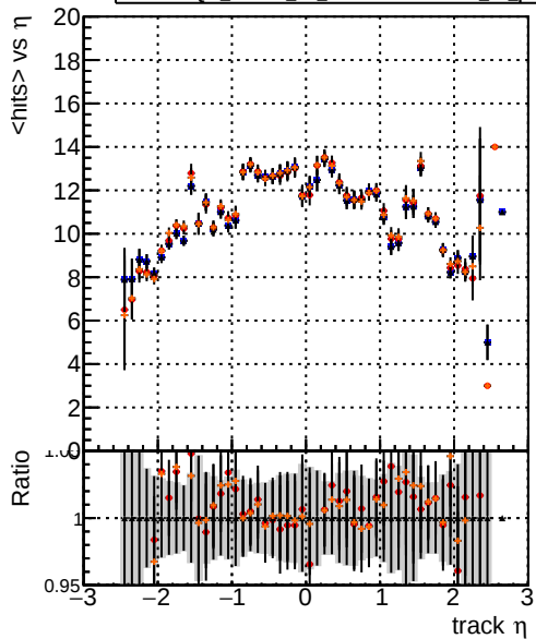
mean hits vs \eta DQM_mkFit5_TT_retrainOldFiles125_v2_prelimWP_epoch4 DQM_mkFit5_TT_baseline_6iter DQM_mkFit6_TT_retrainOldFiles125_v2_prelimWP_epoch2_wsQCD
