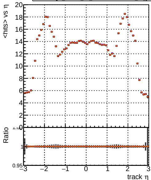
mean hit Legend: - DQM_mkFit_TTbase (blue line) - DQM_mkFit5_TT_retrainOldFiles125_v2_prelimWP_epoch4 (red line with dots) - DQM_mkFit6_TT_retrainOldFiles125_v2_prelimWP_epoch2_wsQCD (orange line with dots)
