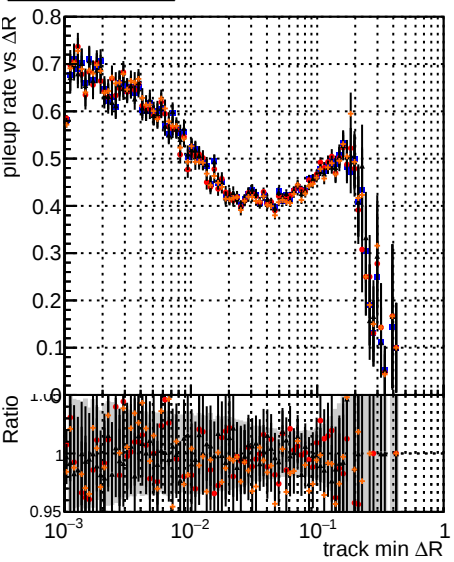
DOM mkFit TTbase retrainOldFiles125_v2_prelimWP_epoch4 DOM mkFit5 TTbase retrainOldFiles125_v2_prelimWP_epoch2 wSQCD DOM mkFit6 TTbase retrainOldFiles125_v2_prelimWP_epoch2 wSQCD
