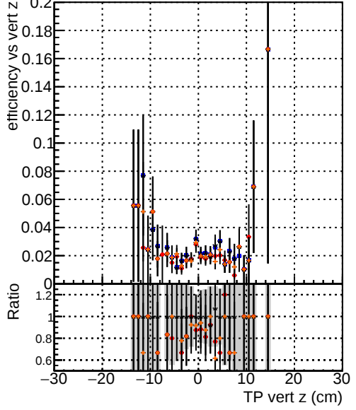
Efficiency vs vertpos DOM_mkFit_TTbase DOM_mkFit5_TT_retrainOldFiles125_v2_prelimWP_epoch4 DOM_mkFit_TT_baseline_6iter DOM_mkFit6_TT_retrainOldFiles125_v2_prelimWP_epoch2_wSQCD
