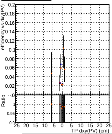
Efficiency vs Dxy(PV) Legend: DQM_mkFit_TTbase DQM_mkFit5_TT_retrainOldFiles125_v2_prelimWP_epoch4 DQM_mkFit_TT_baseline_6iter DQM_mkFit6_TT_retrainOldFiles125_v2_prelimWP_epoch2_wSQCD
