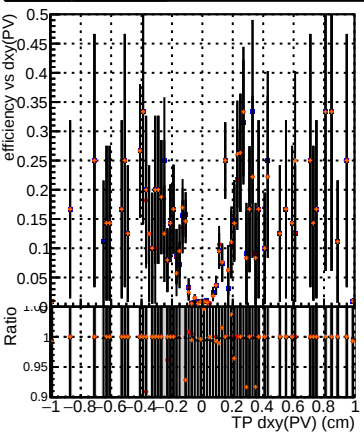
Efficiency vs Dxy(PV) Legend: DQM_mkFit_TTbase DQM_mkFit5_TT_retrainOldFiles125_v2_prelimWP_epoch4 DQM_mkFit_TT_baseline_6iter DQM_mkFit6_TT_retrainOldFiles125_v2_prelimWP_epoch2_wSQCD
