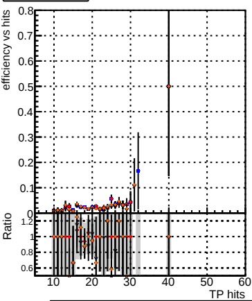
Efficiency vs hit Legend: DQM_mkFit_TTbase DQM_mkFit5_TT_retrainOldFiles125_v2_prelimWP_epoch4 DQM_mkFit_TT_baseline_6iter DQM_mkFit6_TT_retrainOldFiles125_v2_prelimWP_epoch2_wSQCD
