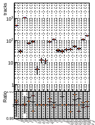
N of reco track vs. \chi^2 for BSM model 125 v2 preliminary WP epoch 4, BSM model 125 v2 preliminary WP epoch 2, and BSM model 125 v2 preliminary WP epoch 2 wSQCD
