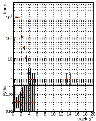
N of reco track vs. \chi^2 for BSM model 125 v2 preliminary WP epoch 4, BSM model 125 v2 preliminary WP epoch 2, and BSM model 125 v2 preliminary WP epoch 2 wSQCD
