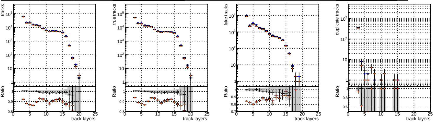
N of reco track vs hit N of associated (recoToSim) tracks vs hit fake tracks N of associated (recoToSim) duplicate tracks vs hit DOM mknet15 TTbase DOM mknet15 TTbase DOM mknet15 TTbase DOM mknet15 TTbase retrainOldFiles125 v2 prelimWP epoch4 retrainOldFiles125 v2 prelimWP epoch2 wSQCD
