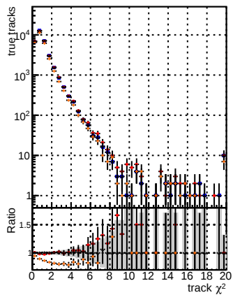
N of reco track vs. \chi^2 for BSM mktFit, BSM mktFit + base, BSM mktFit + base + retrainOldFiles125 v2_prelimWP_epoch4, BSM mktFit + base + retrainOldFiles125 v2_prelimWP_epoch2_wSQCD
