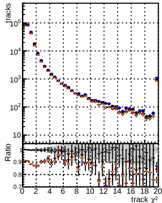
N of reco track vs. \chi^2 for BSM mkt15 + trainOldFiles125 v2_prelimWP_epoch4 (blue), BSM mkt16 + trainOldFiles125 v2_prelimWP_epoch4 (red), and BSM mkt16 + trainOldFiles125 v2_prelimWP_epoch4 wSQCD (black)
