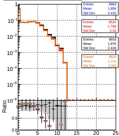
mean hit DOM_mkFit1_TTbase DOM_mkFit5_TT_retrainOldFiles125_v2_prelimWP_epoch4 DOM_mkFit6_TT_retrainOldFiles125_v2_prelimWP_epoch2_wSQCD
