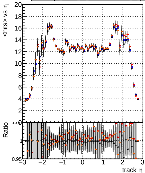
mean hit DOM_mkFit1_TTbase DOM_mkFit5_TT_retrainOldFiles125_v2_prelimWP_epoch4 DOM_mkFit6_TT_retrainOldFiles125_v2_prelimWP_epoch2_wSQCD
