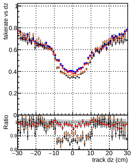
Legend: - \text{DQM\_mkFit\_TTbase} (black line) - \text{DQM\_mkFit\_TTbase\_trainOldFiles125\_v2\_prelimWP\_epoch4} (blue line) - \text{DQM\_mkFit\_TTbase\_trainOldFiles125\_v2\_prelimWP\_epoch2\_wSQCD} (orange line) - \text{DQM\_mkFit\_TTbase\_trainOldFiles125\_v2\_prelimWP\_epoch2\_wSQCD} (red line)
