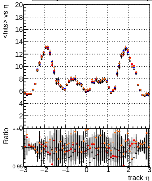
mean hits DOM_mkFit1_TTbase DOM_mkFit5_TT_retrainOldFiles125_v2_prelimWP_epoch4 DOM_mkFit6_TT_retrainOldFiles125_v2_prelimWP_epoch2_wsQCD
