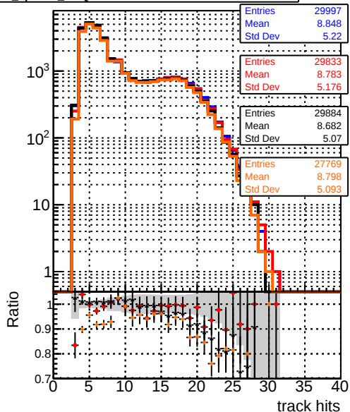
mean hits DOM_mkFit1_TTbase DOM_mkFit5_TT_retrainOldFiles125_v2_prelimWP_epoch4 DOM_mkFit6_TT_retrainOldFiles125_v2_prelimWP_epoch2_wsQCD
