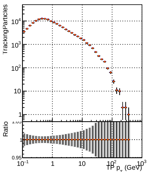
—•— DQM_mkFit1_TTbase —•— DQM_mkFit5_TT_retrainOldFiles125_v2_prelimWP_epoch4 —•— DQM_mkFit6_TT_baseline_6iter —•— DQM_mkFit6_TT_retrainOldFiles125_v2_prelimWP_epoch2_wsQCD
