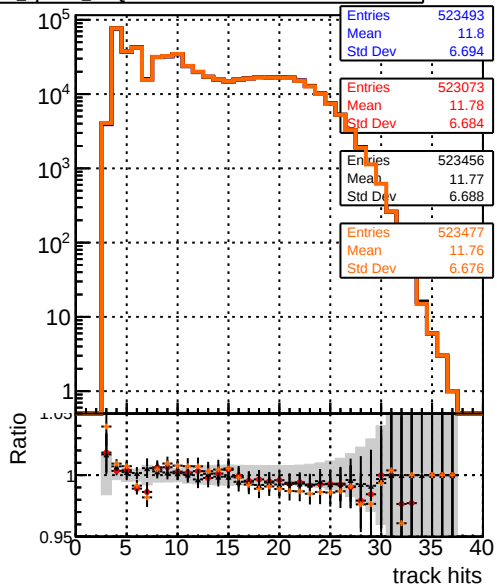
— DQM_mkFit6_TT_base — DQM_mkFit5_TT_retrainOldFiles125_v2_prelimWP_epoch4 — DQM_mkFit6_TT_base_line_6iter — DQM_mkFit6_TT_retrainOldFiles125_v2_prelimWP_epoch2_wSQCD mean hit
