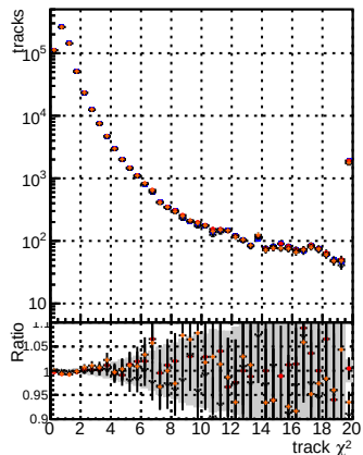
N of reco track vs. \chi^2 for different models and training sets
