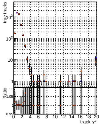
N of reco track vs. \chi^2 for BSM mFit TTbase, BSM mFit TTbase + ttTrainOldFiles125 v2 prelimWP_epoch4, BSM mFit TTbase + ttTrainOldFiles125 v2 prelimWP_epoch2 wSQCD
