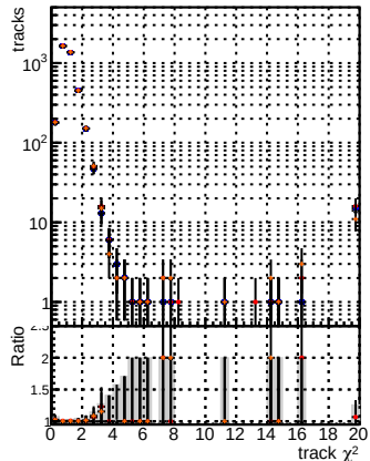
N of reco track vs. \chi^2 for BSM mFit TTbase, BSM mFit TTbase + ttTrainOldFiles125 v2 prelimWP_epoch4, BSM mFit TTbase + ttTrainOldFiles125 v2 prelimWP_epoch2 wSQCD
