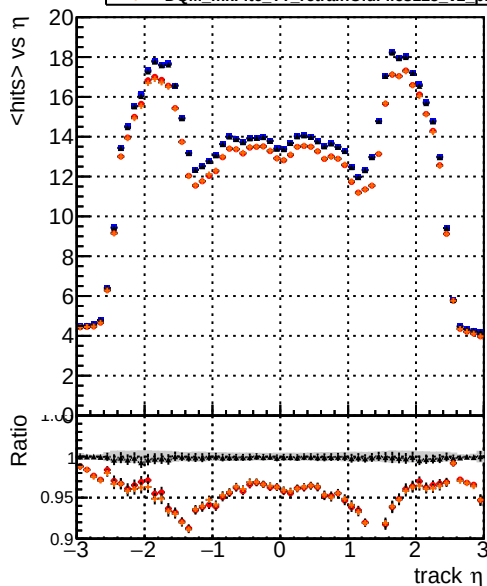
Legend: DQM_mkFit5_TTbase (blue line), DQM_mkFit5_TT_retrainOldFiles125_v2_prelimWP_epoch4 (red line), DQM_mkFit6_TT_baseLine_6iter (black line), DQM_mkFit6_TT_retrainOldFiles125_v2_prelimWP_epoch2_wSQCD (orange line) mean hits > \eta
