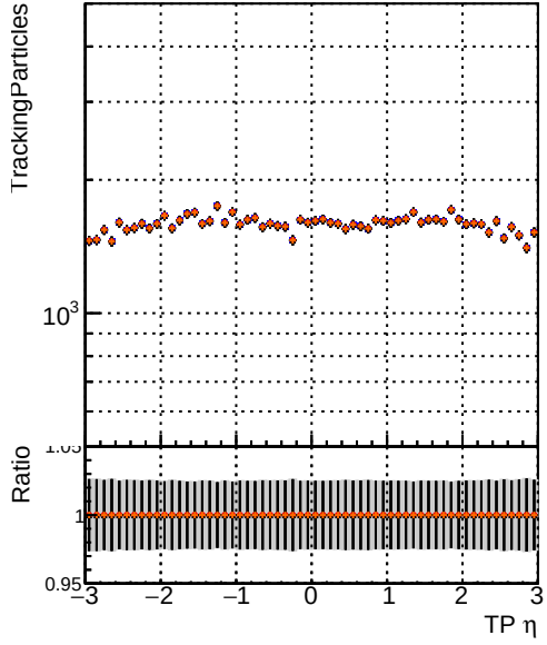
N of simulated tracks vs \eta Legend: DQM_mkFit_TTbase DQM_mkFit5_TT_retrainOldFiles125_v2_prelimWP_epoch4 DQM_mkFit_TT_baseline_6iter DQM_mkFit6_TT_retrainOldFiles125_v2_prelimWP_epoch4
