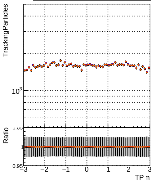
N of simulated tracks vs \eta Legend: QOM_mkFit6_TT_retrainOldFiles125_v2_prelimWP_epoch4 QOM_mkFit5_TT_retrainOldFiles125_v2_prelimWP_epoch4 QOM_mkFit6_TT_retrainOldFiles125_v2_prelimWP_epoch4 QOM_mkFit6_TT_retrainOldFiles125_v2_prelimWP_epoch4
