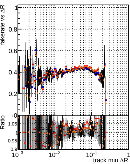
DOM mkFit TTbase retrainOldFiles125_v2_prelimWP_epoch4 DOM mkFit5 TTbase retrainOldFiles125_v2_prelimWP_epoch4 DOM mkFit6 TTbase retrainOldFiles125_v2_prelimWP_epoch4
