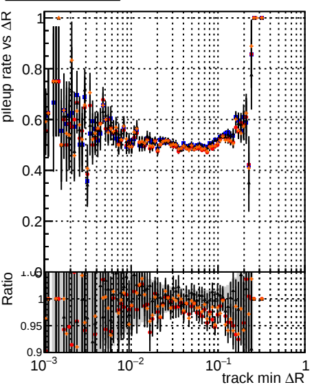
DOM mkFit TTbase retrainOldFiles125_v2_prelimWP_epoch4 DOM mkFit5 TTbase retrainOldFiles125_v2_prelimWP_epoch4 DOM mkFit6 TTbase retrainOldFiles125_v2_prelimWP_epoch4
