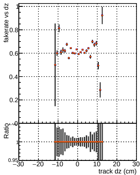
Fake rate vs d DOM mkFit TTbase DOM mkFit5 TTbase DOM mkFit6 TTbase
