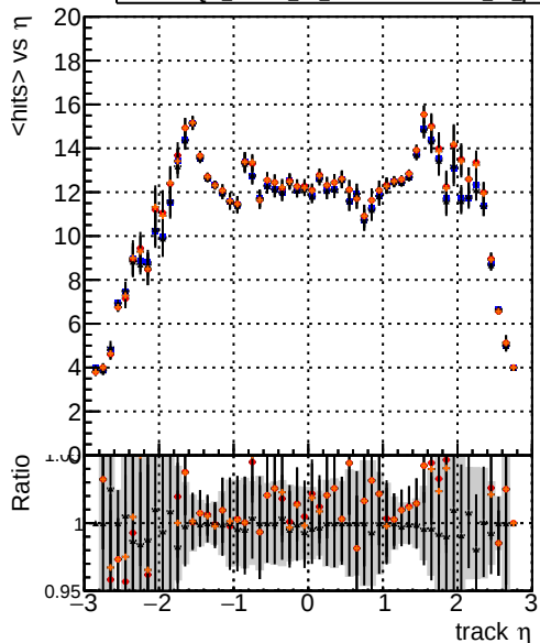
mean hits vs \eta Legend: - DQM_mkFit5_TT_base (blue line with circles) - DQM_mkFit5_TT_retrainOldFiles125_v2_prelimWP_epoch4 (red line with circles) - DQM_mkFit6_TT_base (black line with circles) - DQM_mkFit6_TT_retrainOldFiles125_v2_prelimWP_epoch4 (orange line with circles)
