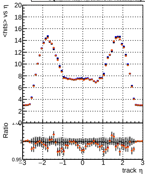
Legend: DQM_mkFit5_TTbase (blue line), DQM_mkFit5_TT_retrainOldFiles125_v2_prelimWP_epoch4 (red line with dots), DQM_mkFit6_TT_baseLine_6iter (black line with dots), DQM_mkFit6_TT_retrainOldFiles125_v2_prelimWP_epoch4 (orange line with dots). mean hits > \eta
