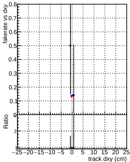
Fake rate vs d Legend: DGM-mkFit-TTbase (Blue line with circles) DGM-mkFit-TT-retrainOldFiles125_v2_prelimWP_epoch4 (Red line with circles) DGM-mkFit6-TT-baselineOldFiles125_v2_prelimWP_epoch4 (Black line with circles) d DGM-mkFit-TTbase DGM-mkFit-TT-retrainOldFiles125_v2_prelimWP_epoch4 DGM-mkFit6-TT-baselineOldFiles125_v2_prelimWP_epoch4 0 0.0 0.0 0.0 1 0.0 0.0 0.0 2 0.0 0.0 0.0 3 0.0 0.0 0.0 4 0.0 0.0 0.0 5 0.0 0.0 0.0 6 0.0 0.0 0.0 7 0.0 0.0 0.0 8 0.0 0.0 0.0 9 0.0 0.0 0.0 10 1.0 1.0 1.0
