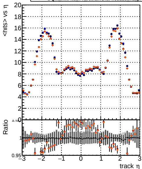
mean hits vs \eta Legend: DQM_mkFit1_TTbase DQM_mkFit5_TT_retrainOldFiles125_v2_prelimWP_epoch4 DQM_mkFit6_TT_baseline_6iter DQM_mkFit6_TT_retrainOldFiles125_v2_prelimWP_epoch4
