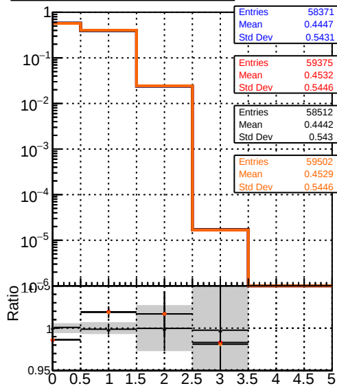
mean hits vs \eta Legend: DQM_mkFit1_TTbase DQM_mkFit5_TT_retrainOldFiles125_v2_prelimWP_epoch4 DQM_mkFit6_TT_baseline_6iter DQM_mkFit6_TT_retrainOldFiles125_v2_prelimWP_epoch4
