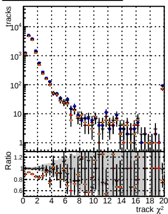
N of reco track vs. \chi^2 for BSM mFit TTbase, BSM mFit TTbase + L1, and BSM mFit TTbase + L1 + L2. The legend indicates the models used in the plots.
