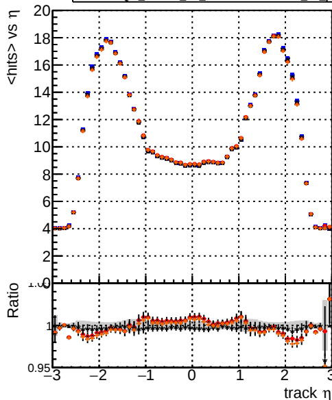
Legend: DQM_mkFit6_TTbase (blue), DQM_mkFit5_TT_retrainOldFiles125_v2_prelimWP_epoch4 (red), DQM_mkFit6_TT_baseline_6iter (black), DQM_mkFit5_TT_retrainOldFiles125_v2_prelimWP_epoch4 (orange) mean hit
