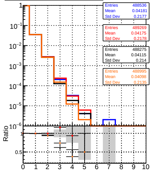
Legend: DQM_mkFit6_TTbase (blue), DQM_mkFit5_TT_retrainOldFiles125_v2_prelimWP_epoch4 (red), DQM_mkFit6_TT_baseline_6iter (black), DQM_mkFit5_TT_retrainOldFiles125_v2_prelimWP_epoch4 (orange) mean hit
