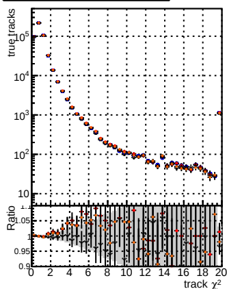
N of reco track vs. \chi^2 for BSM mFit TTbase, BSM mFit TTbase + 11 base, BSM mFit TTbase + 11 + 125 v2 prelimWP epoch4
