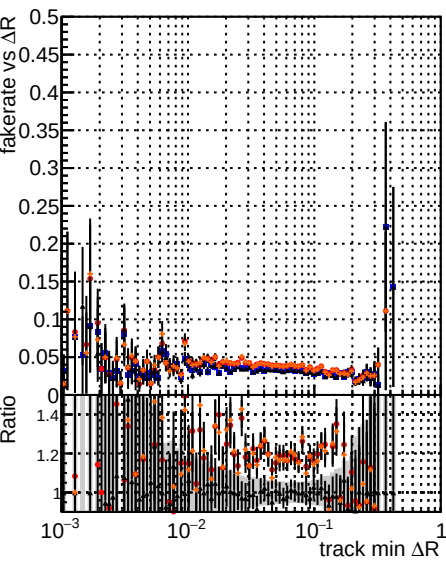
Fake rate vs \Delta R(\text{track, jet}) DOM mkFit TTbase retrainOldFiles125 v2 prelimWP epoch4 DOM mkFit TT baseline epoch4 DOM mkFit6 TT retrainOldFiles125 v2 prelimWP epoch4
