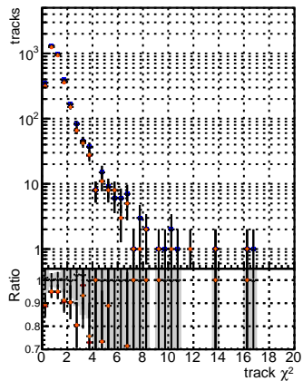
N of reco track vs. \chi^2 for BDM mkFit v2 (blue circles), BDM mkFit v2 (orange circles), and BDM mkFit v2 (grey circles). The legend also includes BDM mkFit v2 (blue circles), BDM mkFit v2 (orange circles), and BDM mkFit v2 (grey circles).
