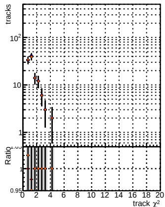
N of reco track vs. \chi^2 for BSM mFit TTrees, BSM mFit TTrees + Lb, BSM mFit TTrees + Lb + baseline SF
