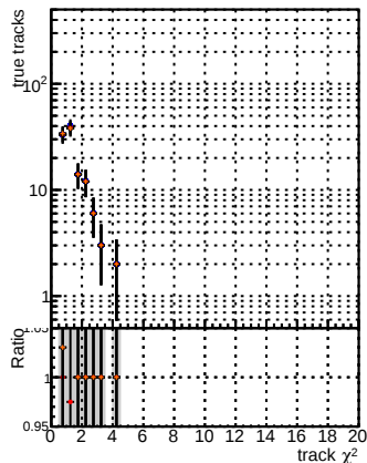
N of reco track vs. \chi^2 for BSM mFit TTrees, BSM mFit TTrees + Lb, BSM mFit TTrees + Lb + baseline SF
