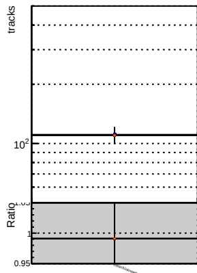
N of reco track vs. \chi^2 for BSM mFit TTrees, BSM mFit TTrees + Lb, BSM mFit TTrees + Lb + baseline SF
