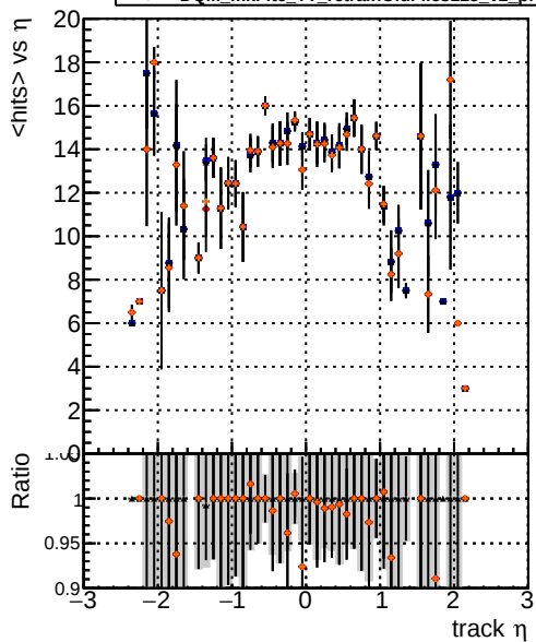
mean hits vs \eta Legend: - DQM_mkFit5_TT_base (blue line with circles) - DQM_mkFit5_TT_retrainOldFiles125_v2_prelimWP_epoch4 (red line with circles) - DQM_mkFit6_TT_base (black line with circles) - DQM_mkFit6_TT_retrainOldFiles125_v2_prelimWP_epoch4 (orange line with circles)
