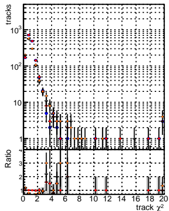
N of reco track vs. \chi^2 for BDM mkFit v2 (blue circles), BDM mkFit v2 (orange circles), and BDM mkFit v2 (red circles). The legend also includes 'BDM mkFit v2' and 'BDM mkFit v2'.
