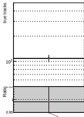
N of reco track vs. \chi^2 for BSM mF F T base and BSM mF F T train OldFiles125 v2_prelimWP_epoch4
