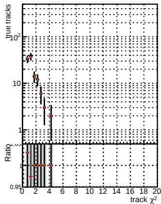
N of reco track vs. \chi^2 for BSM mF F T base and BSM mF F T train OldFiles125 v2_prelimWP_epoch4
