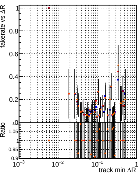
Fake rate vs \Delta R (track, jet) DOM mkFit TT base DOM mkFit TT retrainOldFiles125 v2 prelimWP epoch4 DOM mkFit TT baseline DOM mkFit TT retrainOldFiles125 v2 prelimWP epoch4
