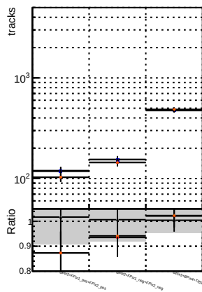
N of reco track vs. \chi^2 for BSM mFit TTbase, BSM mFit TTbase + retrainOldFiles125 v2_prelimWP_epoch4, and BSM mFit TTbase + retrainOldFiles125 v2_prelimWP_epoch4
