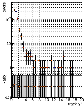
N of reco track vs. \chi^2 for BSM mFit TTbase, BSM mFit TTbase + retrainOldFiles125 v2_prelimWP_epoch4, and BSM mFit TTbase + retrainOldFiles125 v2_prelimWP_epoch4
