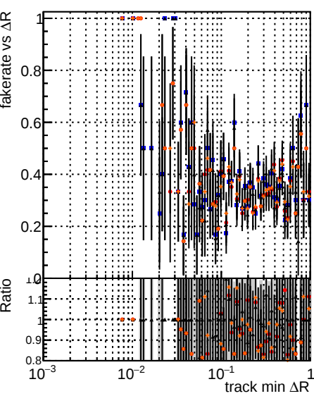
DOM mkFit TTbase DOM mkFit5 TTbase DOM mkFit6 TTbase retrainOldFiles125_v2_prelimWP_epoch4 retrainOldFiles125_v2_prelimWP_epoch4
