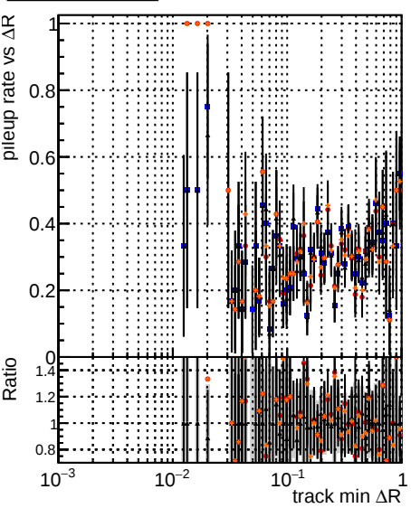
DOM mkFit TTbase DOM mkFit5 TTbase DOM mkFit6 TTbase retrainOldFiles125_v2_prelimWP_epoch4 retrainOldFiles125_v2_prelimWP_epoch4
