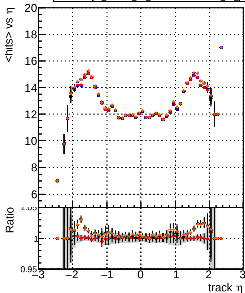
mean hits vs \eta Legend: - DQM_mkFit_TTbase (blue line) - DQM_mkFit5_TT_retrainOldFiles125_v2_prelimWP_epoch4 (red line with dots) - DQM_mkFit_TT_baseline_6iter (black line with dots) - DQM_mkFit6_TT_retrainOldFiles125_v2_prelimWP_epoch4 (orange line with dots)
