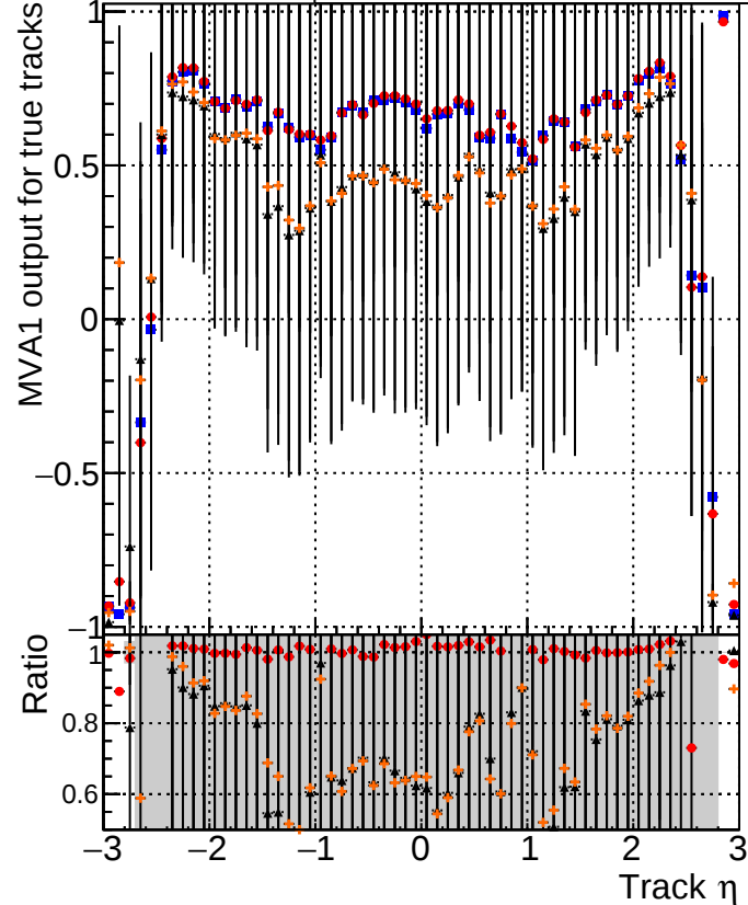
MVA1 of associated tracks (recoToSim) vs. track \eta Legend: — DQM_mkFit_TTbase — DQM_mkFit5_TT_retrainOldFiles125_v2_prelimWP_epoch4 — DQM_mkFit_TT_baseline_6iter — DQM_mkFit6_TT_retrainOldFiles125_v2_prelimWP_epoch4
