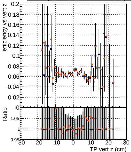
Efficiency vs vert z —●— DQM_mkFit1_TTbase —◆— DQM_mkFit5_TT_retrainOldFiles125_v2_prelimWP_epoch4 —▲— DQM_mkFit6_TT_retrainOldFiles125_v2_prelimWP_epoch4 —×— DQM_mkFit_TT_baseline_6iter Efficiency vs. track reference point z (cm)
