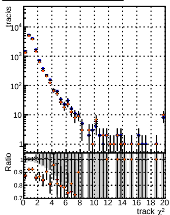
N of reco track vs. \chi^2 for BSM mFit TTbase, BSM mFit TTbase + L1 base and SF, BSM mFit TTbase + L1 + SF, and BSM mFit TTbase + L1 + SF + SF
