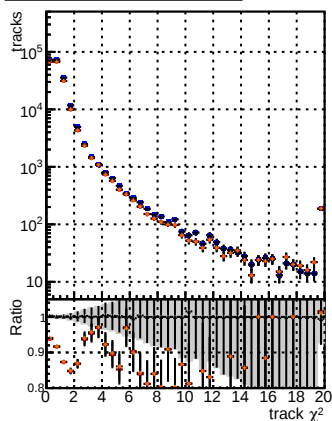
N of reco track vs. \chi^2 for BSM mFit + base + retrain OldFiles125 v2_prelimWP_epoch4
