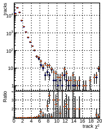
N of reco track vs. \chi^2 for BSM mkFit, TTbase, and BSM mkFit + TTbase. The legend indicates the models used: BSM mkFit, TTbase, and BSM mkFit + TTbase.
