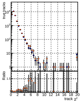
N of reco track vs. \chi^2 for BSM mFit + base, BSM mFit + retrain, and BSM mFit + base + retrain. The legend indicates the methods used for the data points.
