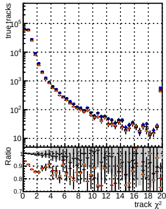
N of reco track vs. \chi^2 for BSM mFit TTbase, BSM mFit TTbase + 11, BSM mFit TTbase + 11 + 125 v2 prelimWP epoch4, BSM mFit TTbase + 11 + 125 v2 prelimWP epoch4 + 125 v2 prelimWP epoch4
