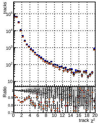
N of reco track vs. \chi^2 for BSM mFit TTbase, BSM mFit TTbase + 11, BSM mFit TTbase + 11 + 125 v2 prelimWP epoch4, BSM mFit TTbase + 11 + 125 v2 prelimWP epoch4 + 125 v2 prelimWP epoch4
